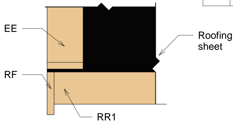
3 Roof Reinforcement
