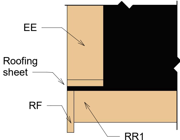
3) Roof Reinforcement
